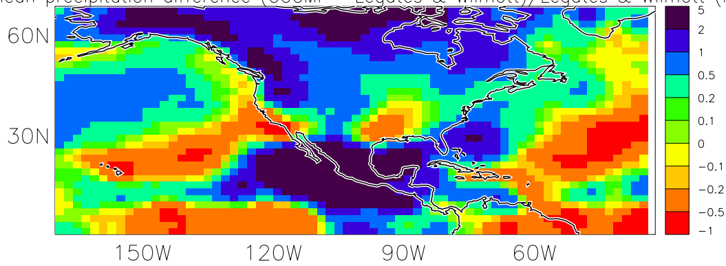
JJA mean precipitation difference (CGCM1 - Legates & Wilmott)/Legates & Wilmott (Frac)
