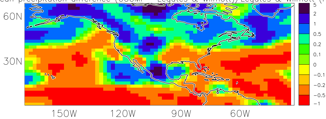
SON mean precipitation difference (CGCM1 - Legates & Wilmott)/Legates & Wilmott (Frac)
