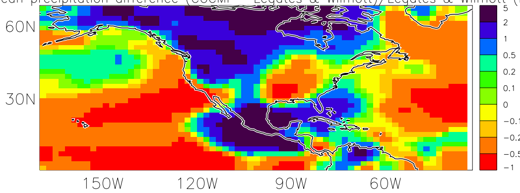
MAM mean precipitation difference (CGCM1 - Legates & Wilmott)/Legates & Wilmott (Frac)
