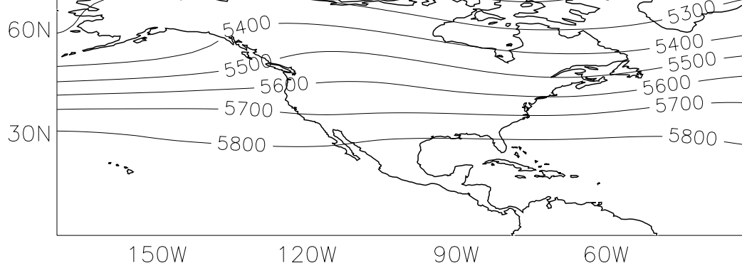
NCEP/NCAR Reanalyses 2x2 JJA mean 500mb Geopotential height (1980-1989) (m)
