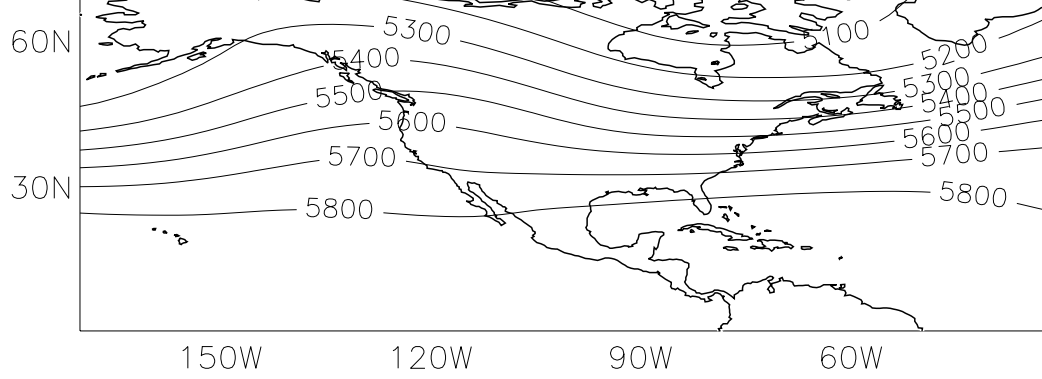
NCEP/NCAR Reanalyses 2x2 MAM mean 500mb Geopotential height (1980-1989) (m)
