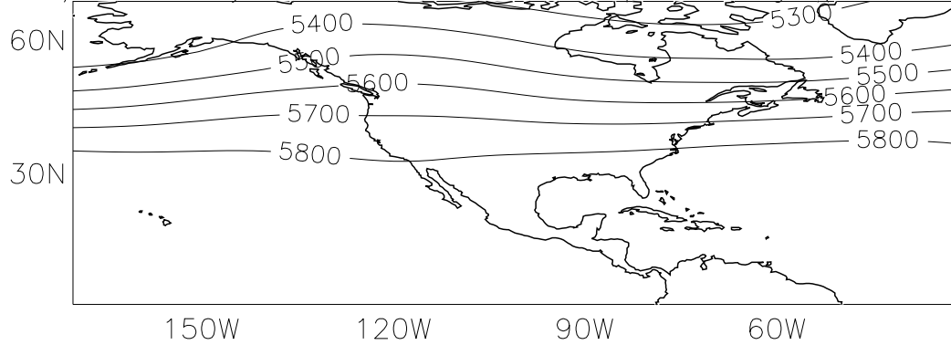
NCEP/NCAR Reanalyses 2x2 SON mean 500mb Geopotential height (1980-1989) (m)
