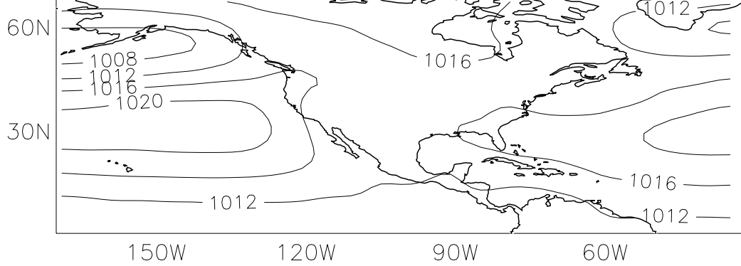
NCEP/NCAR Reanalyses 2x2 JJA mean sea-level pressure (1980-1989) (mb)
