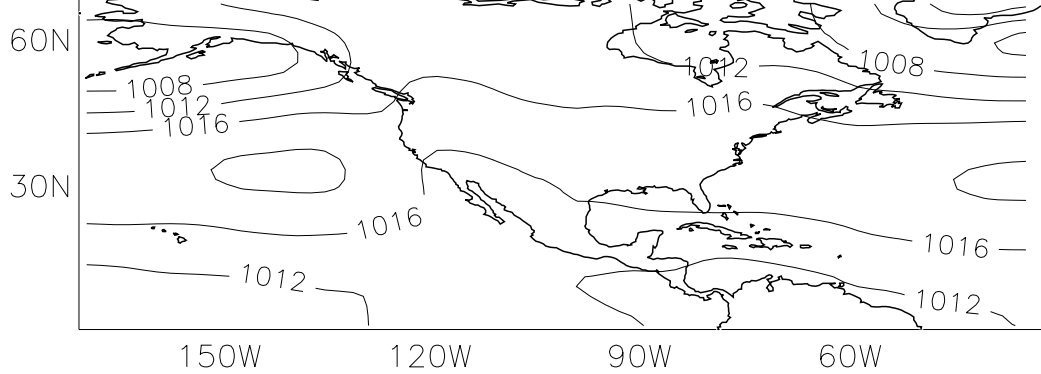
NCEP/NCAR Reanalyses 2x2 SON mean sea-level pressure (1980-1989) (mb)
