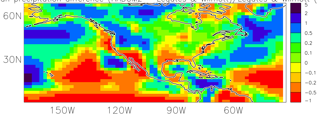
SON mean precipitation difference (HADCM2 - Legates & Wilmott)/Legates & Wilmott (Frac)
