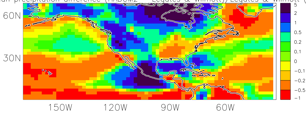
MAM mean precipitation difference (HADCM2 - Legates & Wilmott)/Legates & Wilmott (Frac)
