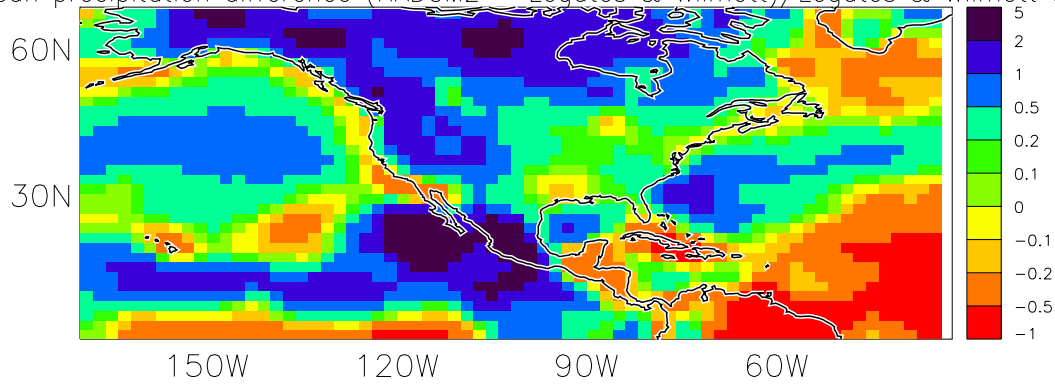
JJA mean precipitation difference (HADCM2 - Legates & Wilmott)/Legates & Wilmott (Frac)
